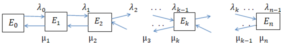
Figure 2. Transition graph of the 'Death and Reproduction' scheme of the switching node of telecommunication networks
