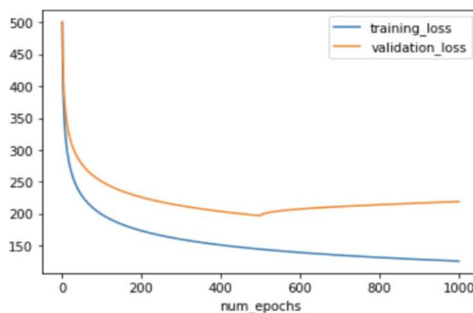
Plot 6: Depiction of "overfitting" during learning.
