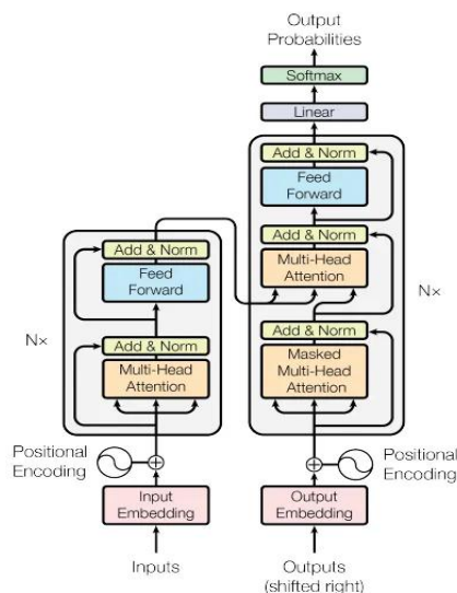
Figure 1. From “Attention is all you need” paper by Anish V., et al., 2017
