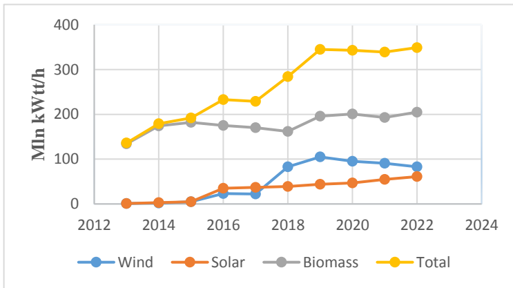
Figure 1. Azerbaijan's renewable energy production in 2013-2022, (Hesabat 2022).
